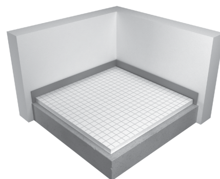
Install the perimeter strip and the Clypso insulation
